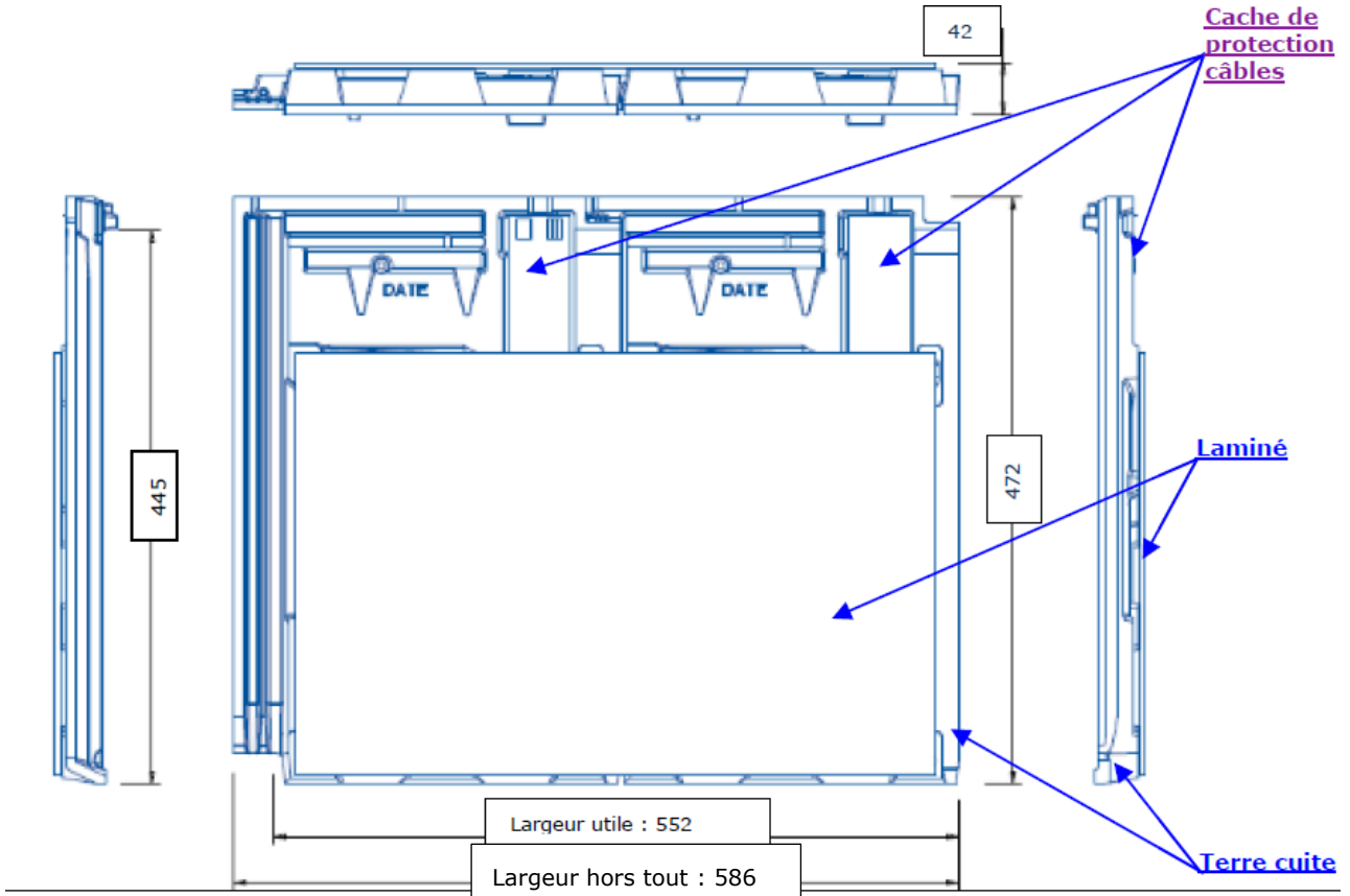
Figure 4 – Support terre cuite Rhôna Solaire
