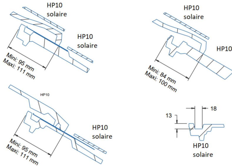
Figure 23 – Recouvrements HP 10 Solaire
