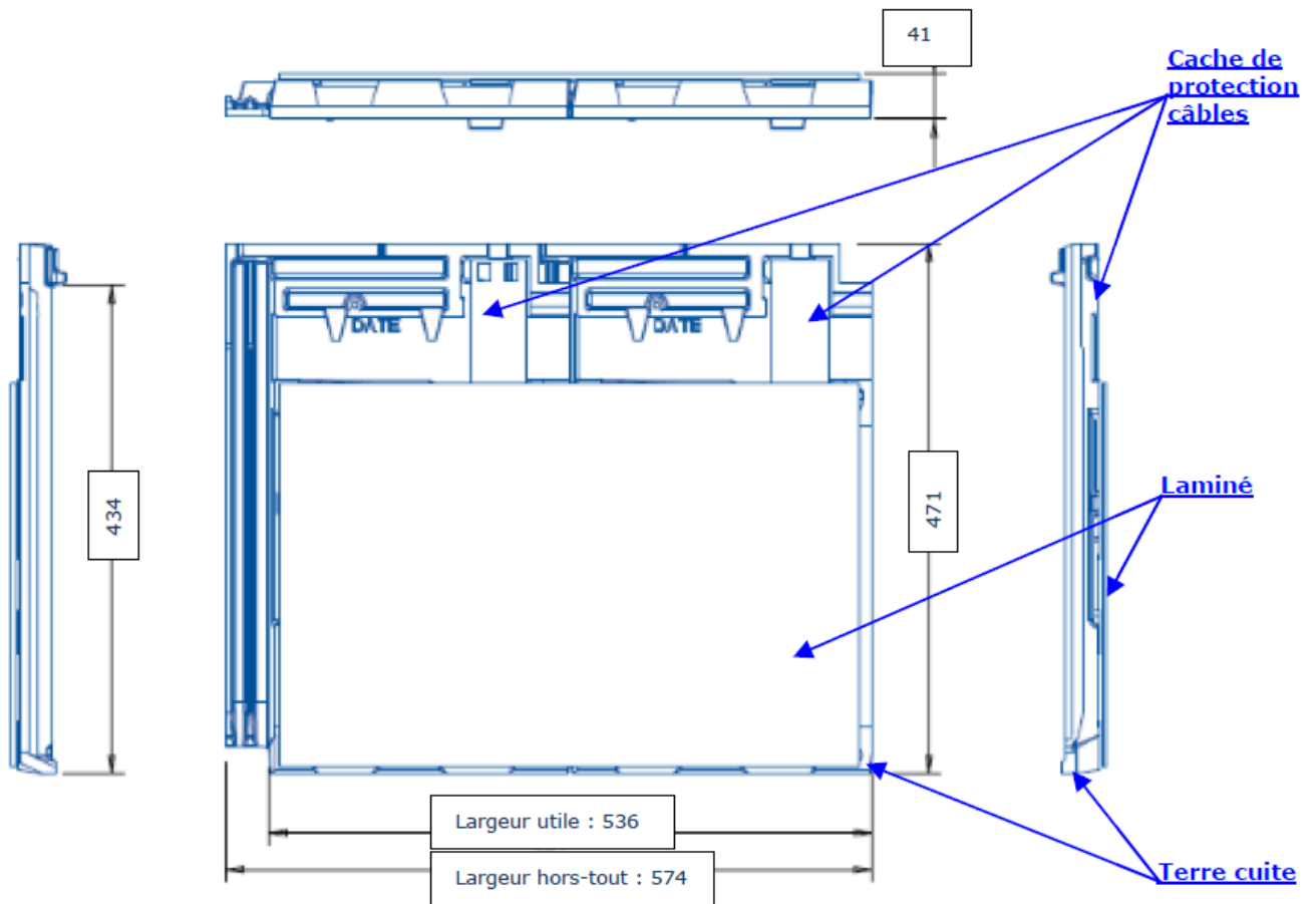
Figure 5 - HP10 Solaire
