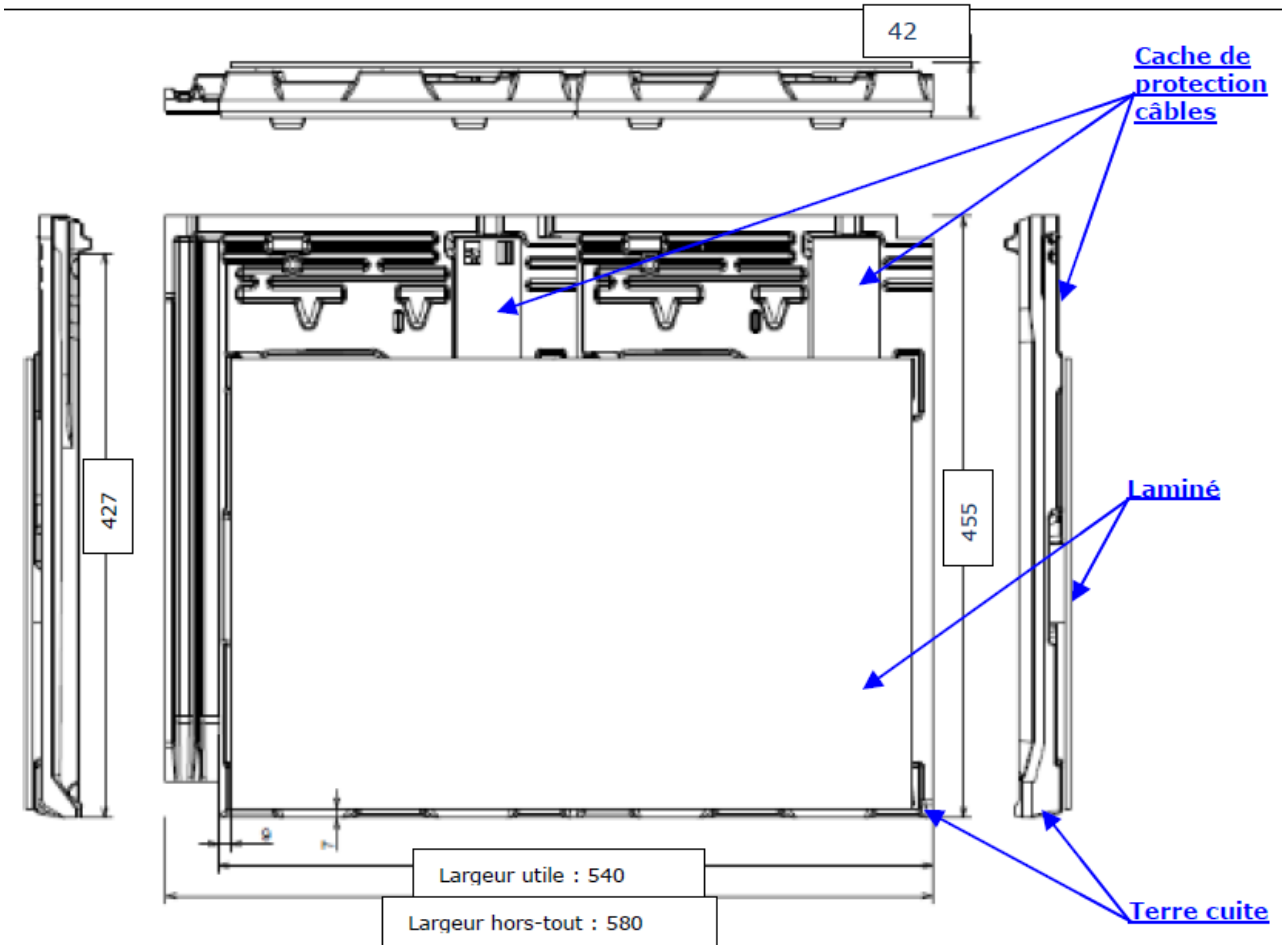
Figure 2 – Support terre cuite Alpha Solaire
