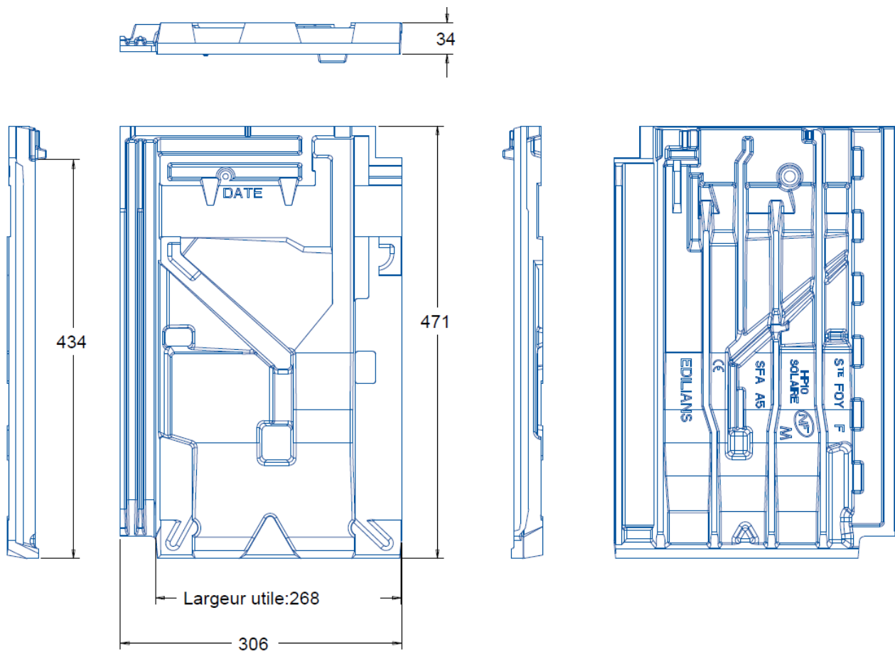
Figure 6 - Support terre cuite HP10 Solaire
