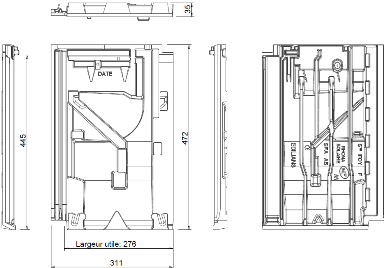
Figure 4 – Support terre cuite Rhôna Solaire
