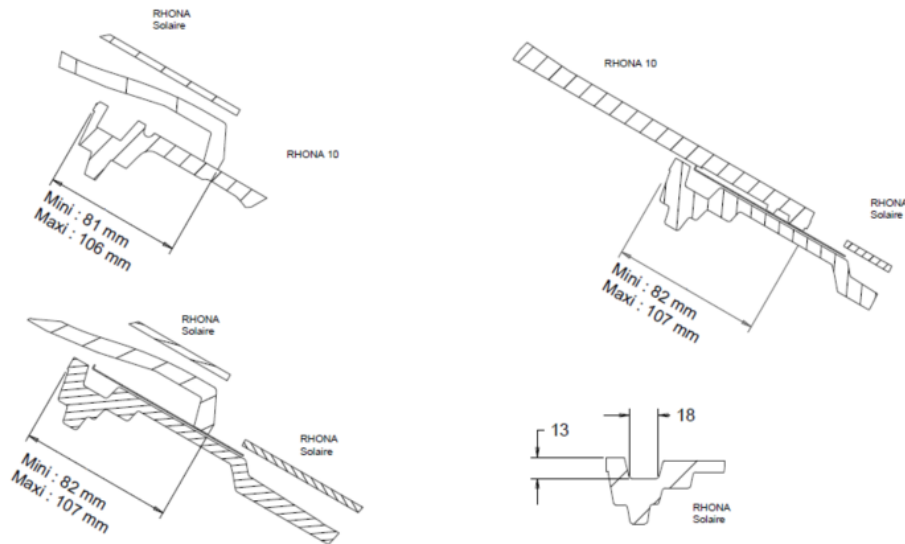
Figure 22 – Recouvrements Rhôna Solaire
