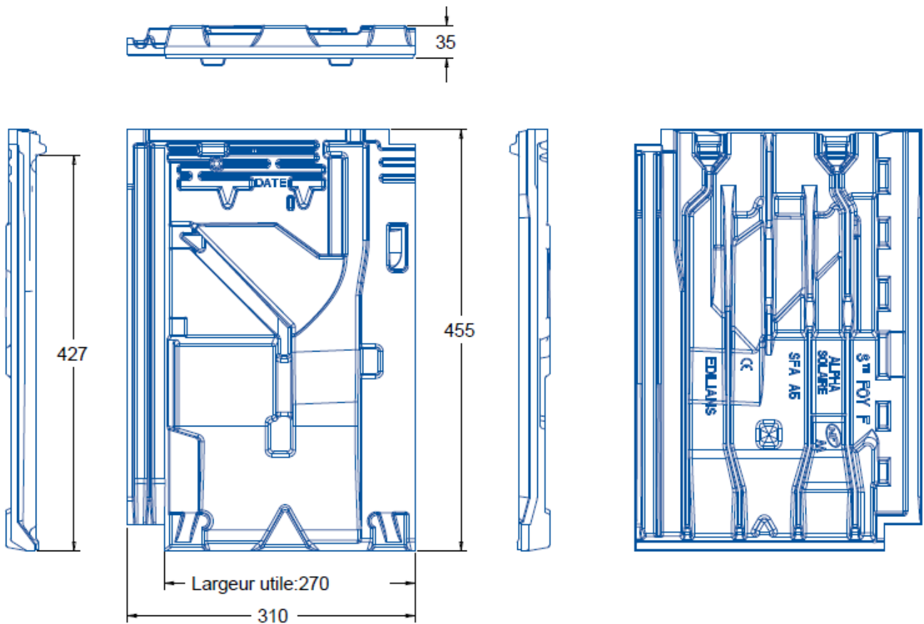
Figure 2 – Support terre cuite Alpha Solaire
