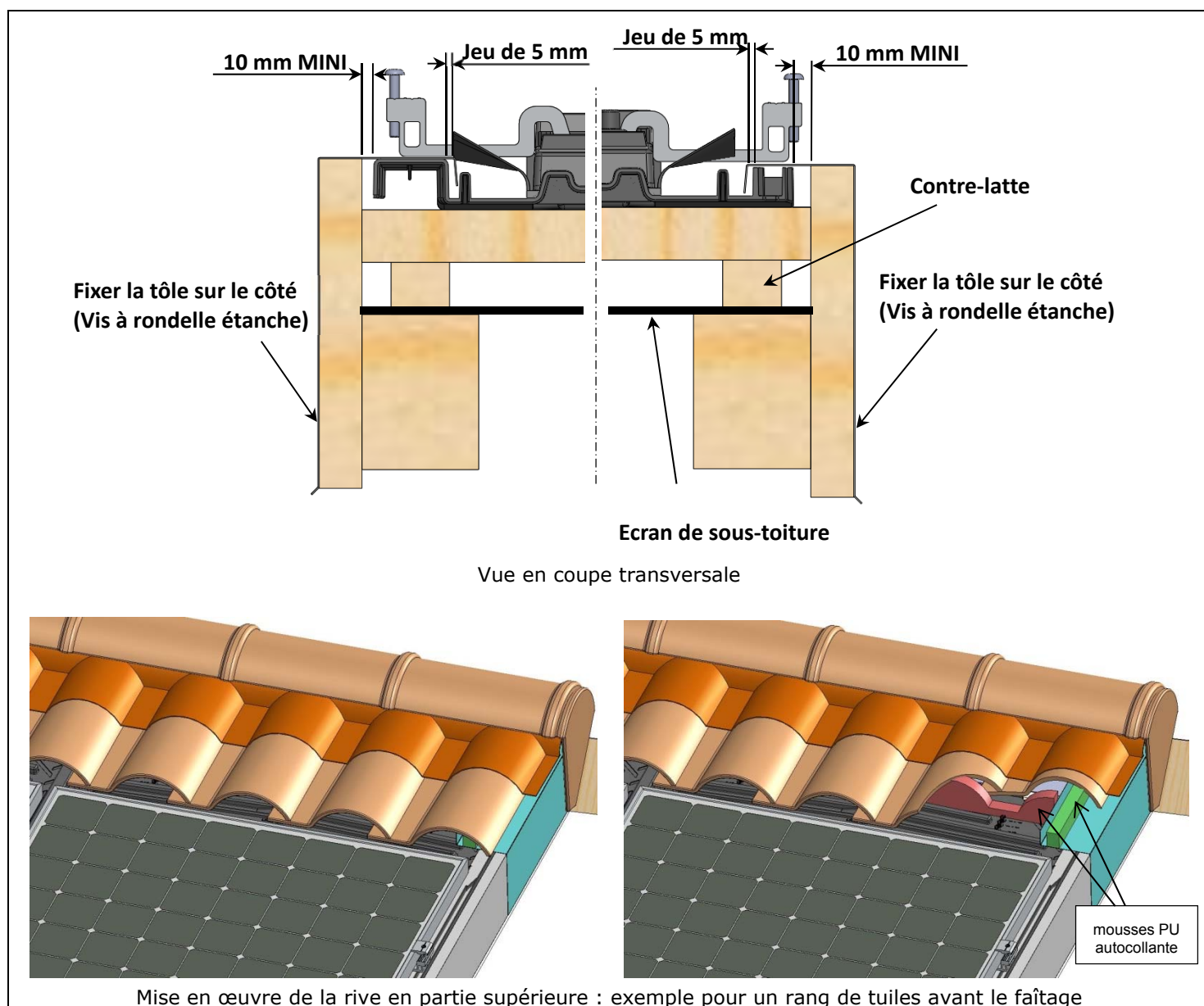
Figure 43 – Pose en rive
