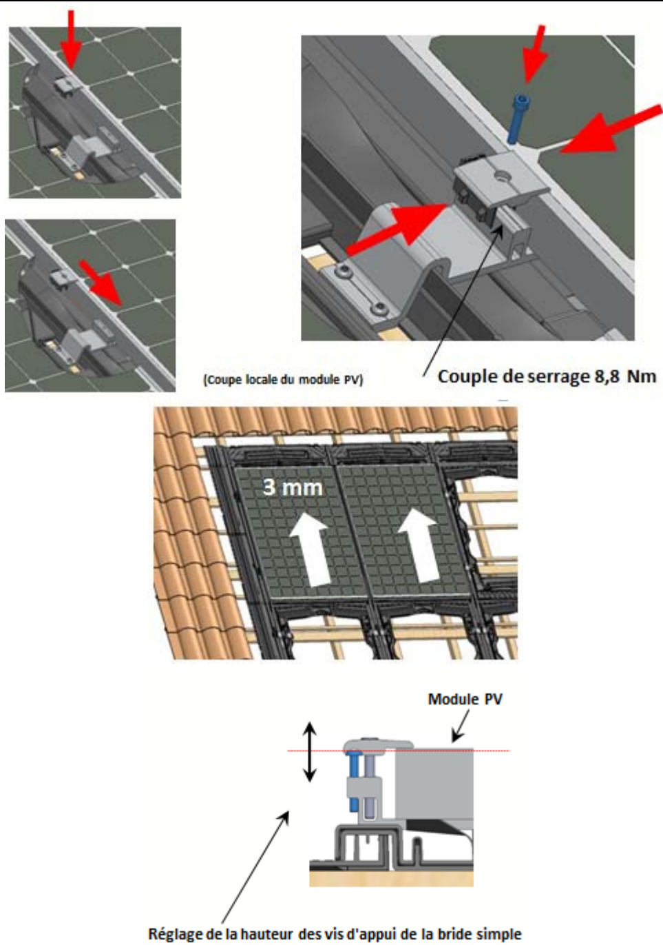
Figure 37 – Pose des modules
