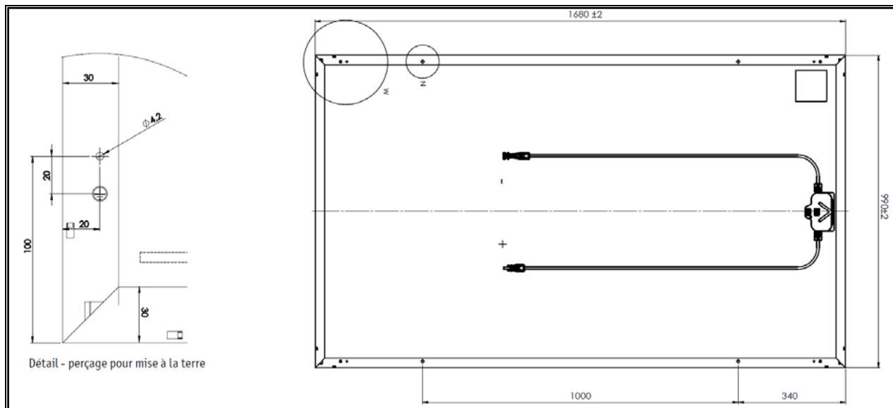
Figure 9 – Module photovoltaïque SolarWatt
