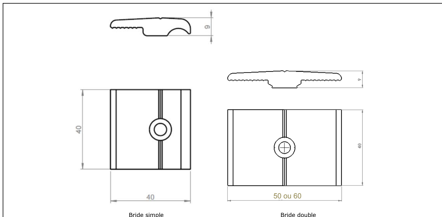
Figure 20 – Brides de fixation Evolution
